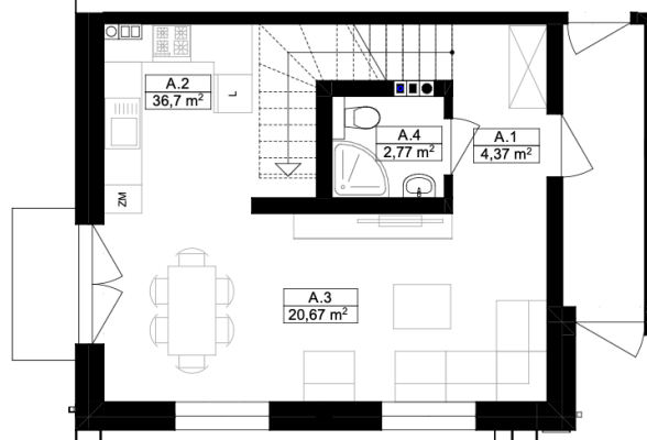
Parter
